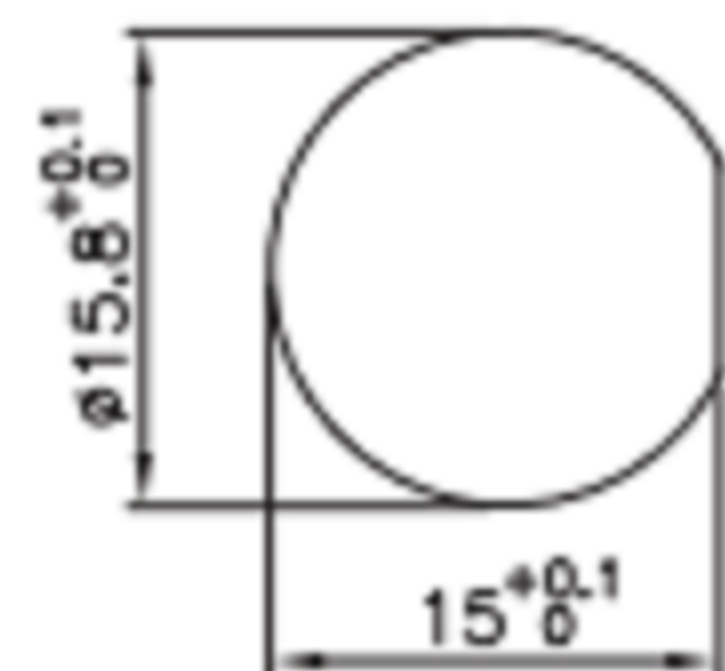
开孔尺寸 hole opening size
